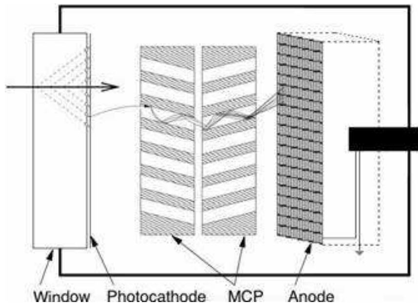
Figure 7: A ‘cartoon’ of a side of a MCP-PMT module, showing the Magnesium-Fluoride window at left, followed by the chevron micro-channel plate, the multi-pad anode, and the pin that penetrates the back of the device to the readout chip. The actual thickness of the module is approximately 1 inch, so the true aspect ratio is more like a tile than this ‘exploded’ view implies. Also shown are an incoming particle making Cherenkov light in the window, and the trajectory of one photo-electron and its shower in the MCP. Typical gains, however, are \sim 10^6 , rather than the small integer depicted in the electron shower.
