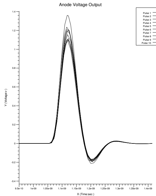
Figure 11: The output voltage from one of the four collectors on the back of the anode for 10 different simulated showers. The simulation includes the frequency response of the generation of Cherenkov light, absorption in the window, the photo-cathode response, the time jitter in the MCP, physical and temporal distributions at the anode, path length differences on the anode, and electrical characteristics of the anode. The RMS jitter on the leading edge as measured at half-height is 0.86 psec.
